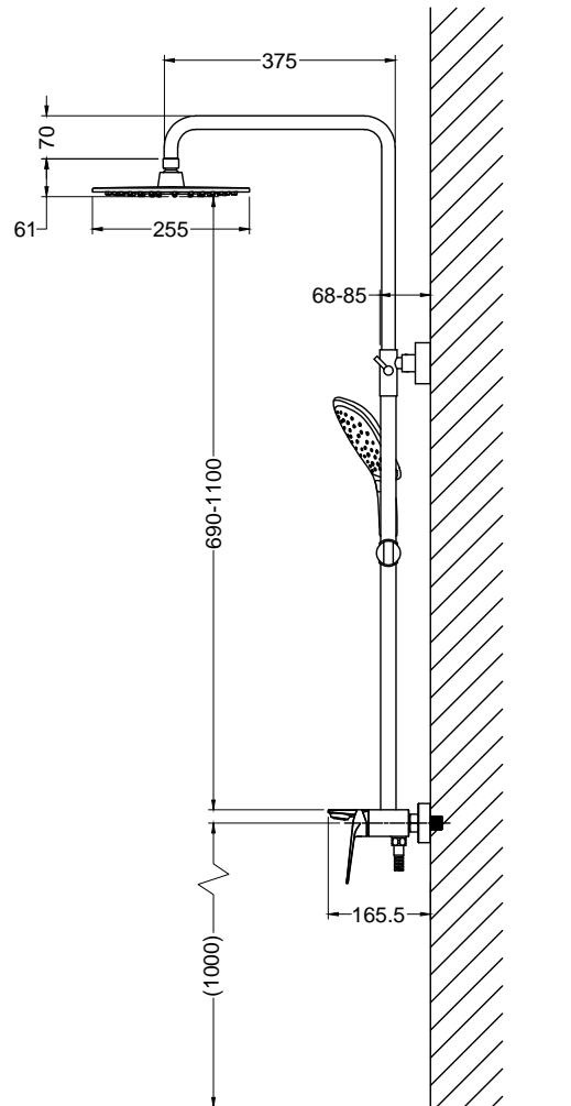
Side view
